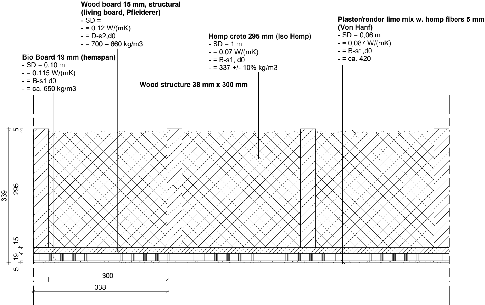
Detail min 15° 1:5
